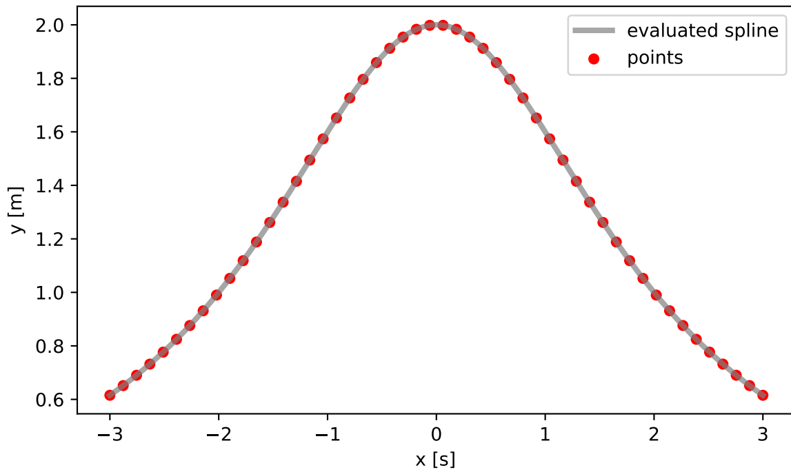
Witch of Agnesi
